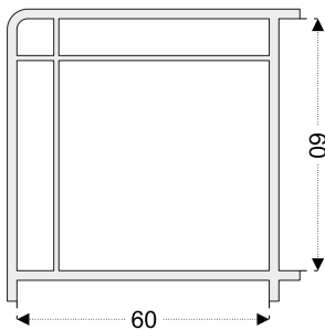
PEN 36 Kutu - 60x60mm (60mm Seri)
