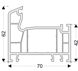
PEN711 Kasa - 42mm
