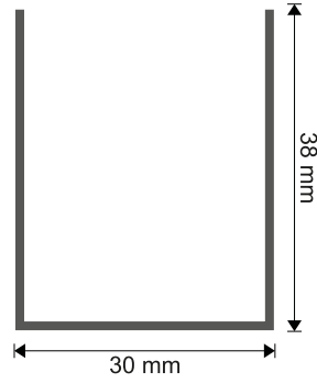
38 x 30 x 38 PEN10, PEN715 PEN716
