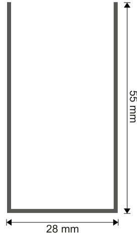
55 x 28 x 55 PEN04
