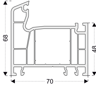
PEN710 Kasa - 48mm
