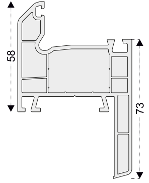
PEN81 Pervazlı Kasa
