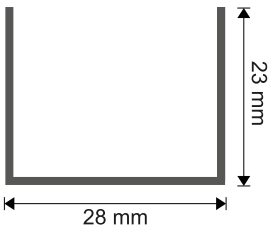
23 x 28 x 23 PEN51, PEN52, PEN53 PEN01, PEN02, PEN03 PEN710, PEN711, PEN712 PEN713, PEN20, PEN21 PEN211
